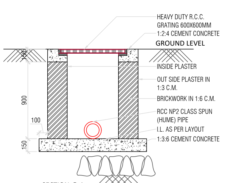
SECTION @ A TYPICAL STORM WATER COLLECTION CHAMBER SCALE 1:25
