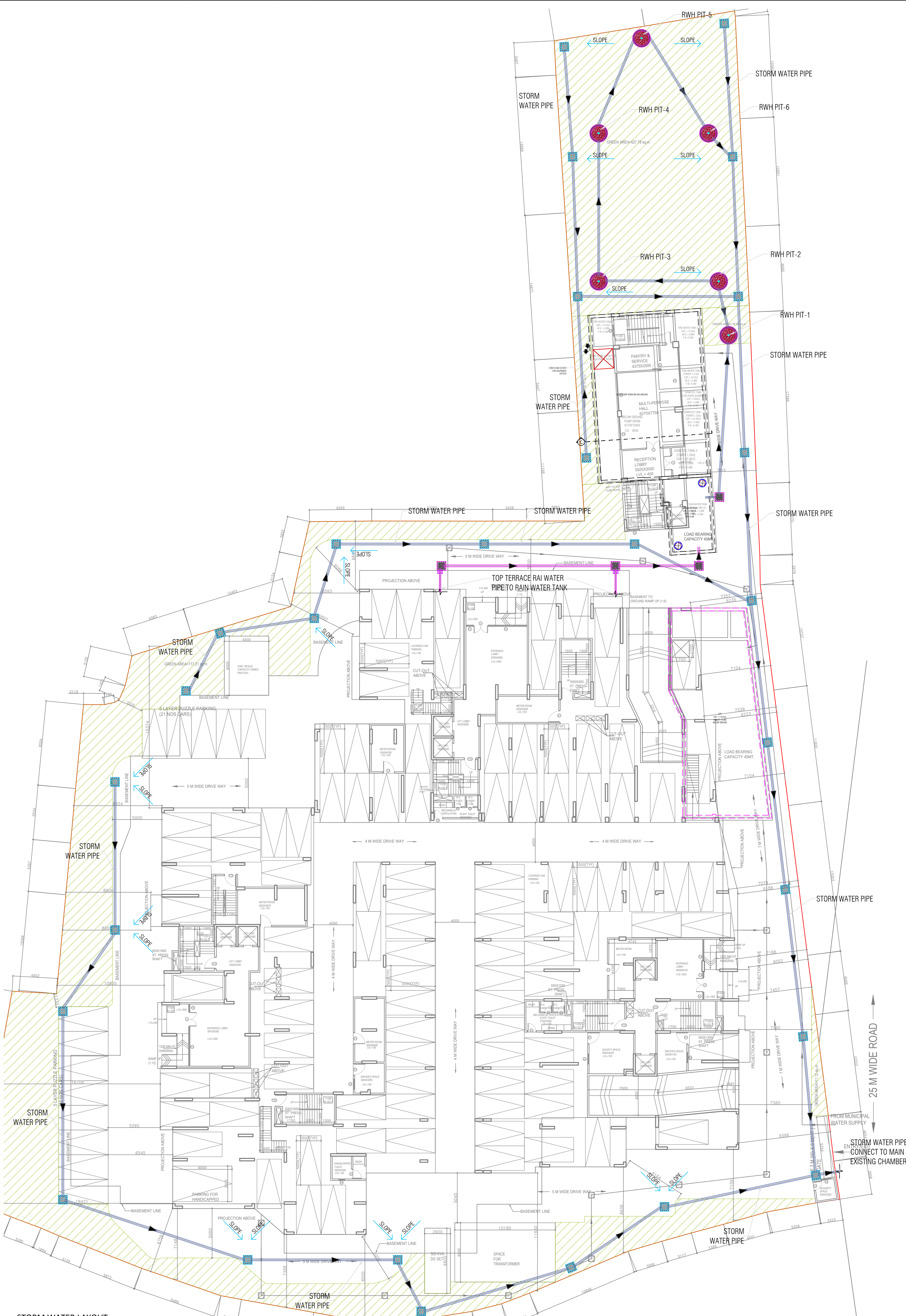
STORM WATER LAYOUT SCALE - 1:200
