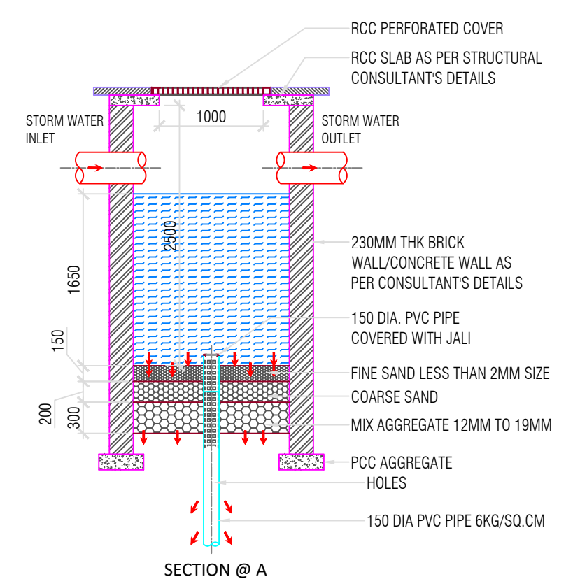
DETAILS FOR TERRACE RAIN WATER RECHARGE PIT (Ø1.5Mx2.5M(D)) SCALE 1:50
